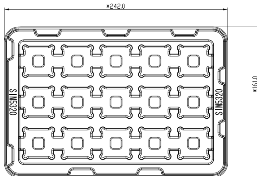
Figure 33: Tray drawing
