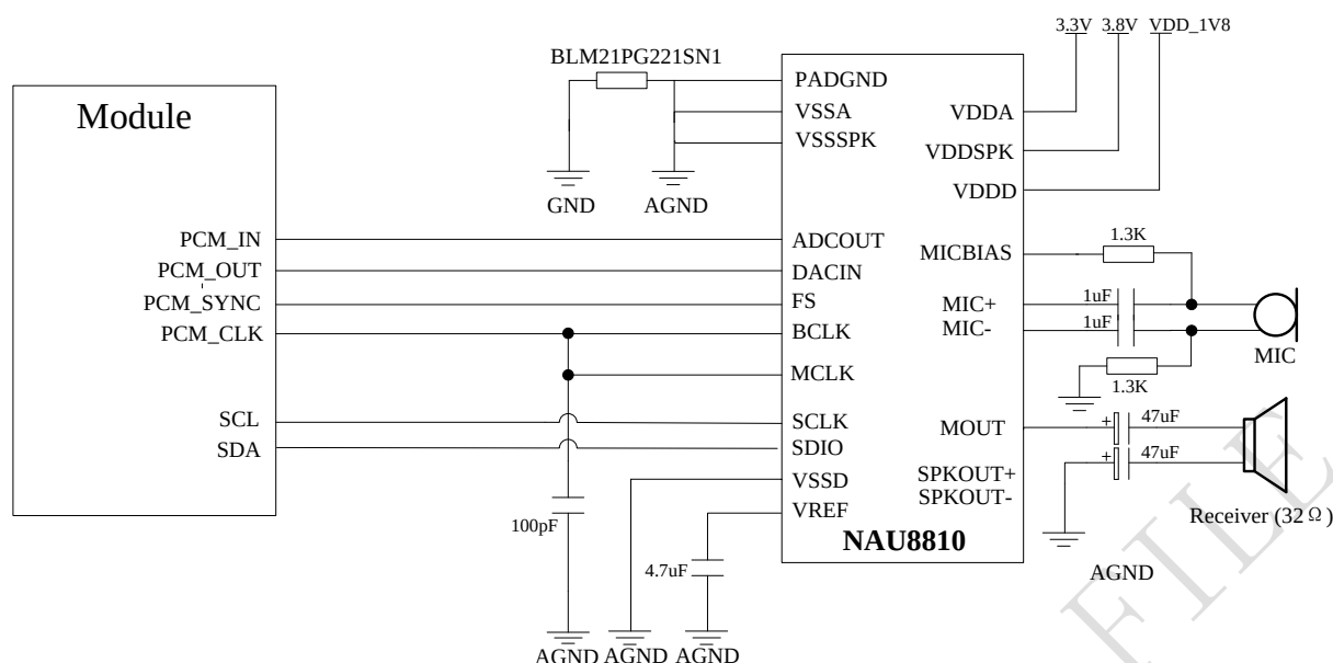
Figure 23: PCM reference circuit
